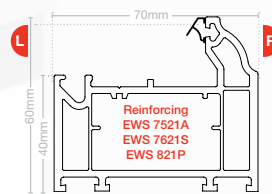
Main frame EWS 7721
