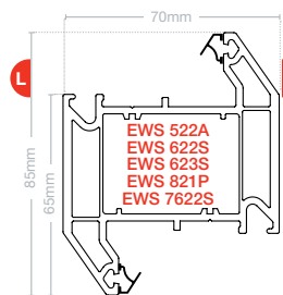
Intermediate transom Z EWS 7023
