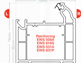
Large main frame EWS 7706
