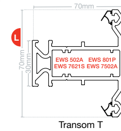
Transom T EWS 7002
