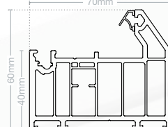
Main frame EWS 7011
